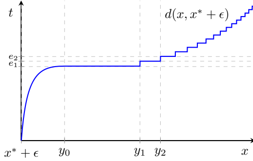
Figure 4: Discontinuous limit solution
